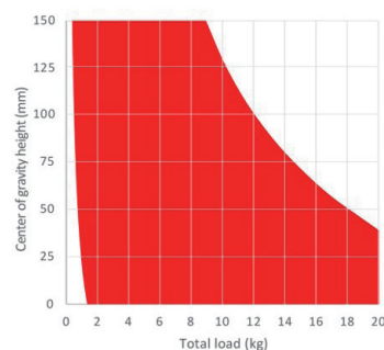
Payload Diagram FSB 10 Mk II
