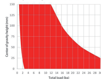
Payload Diagram FSB 14T Mk II
