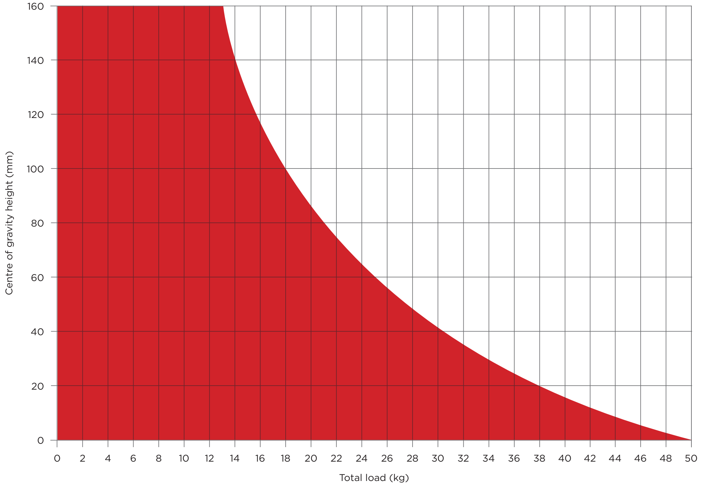
Payload Diagram FSB 18T MK II
