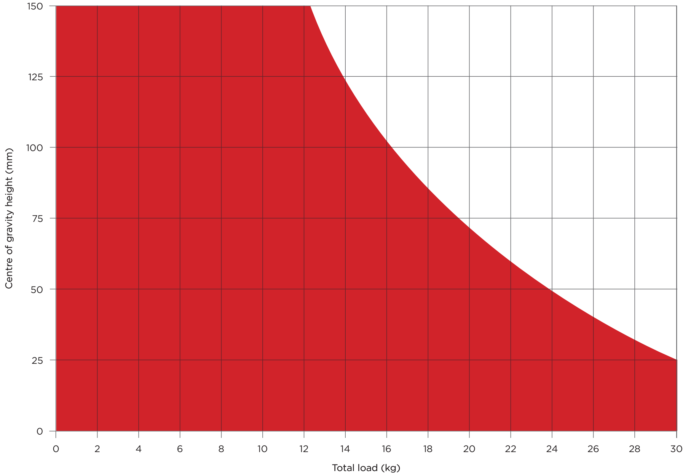
Payload Diagram FSB 16T Mk II
